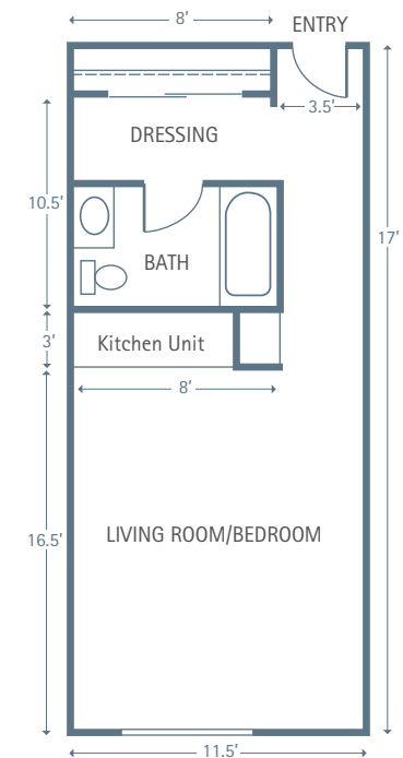
STUDIO APPROXIMATELY 320 SQUARE FEET
