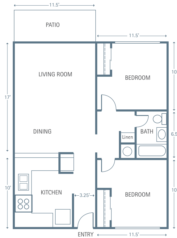
2 BEDROOM APPROXIMATELY 651 SQUARE FEET
